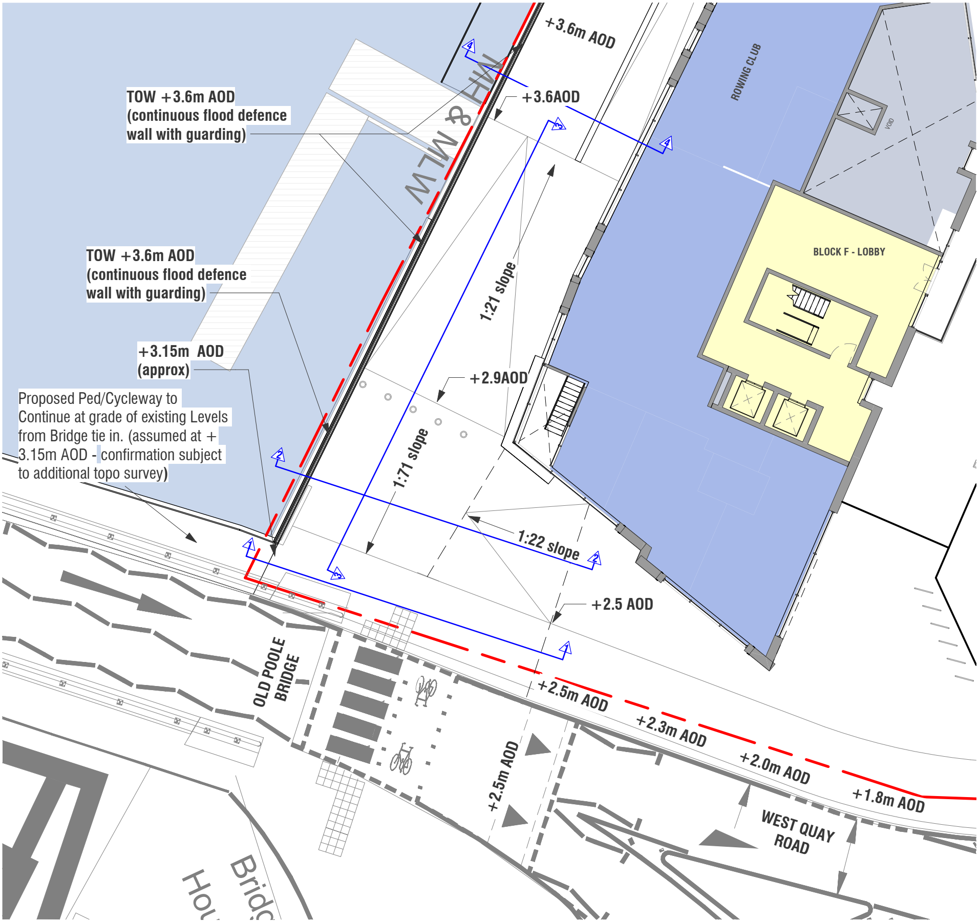
Poole Bridge Quayside Plan
